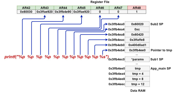
Fig. 3: Overview of the Cross Subroutine Attack.
