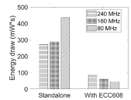
Fig. 16: ECDH energy draw.
