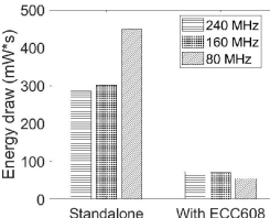
Fig. 15: ECDSA verify energy draw.
